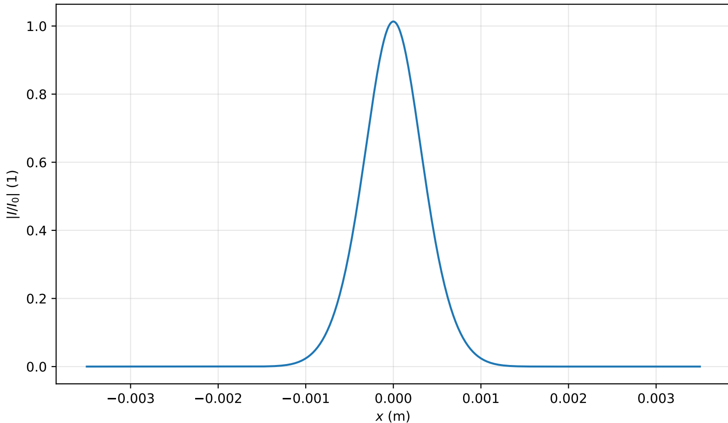
Intensity profile I(x, y = 0, z = 0.796m)/I_0 , P_{in}=0.4P_{cr} , artificial time
